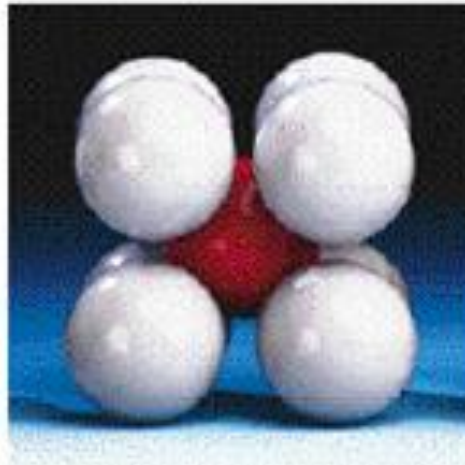
body-centered cubic
