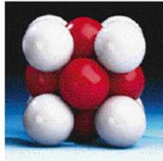
face-centered cubic
